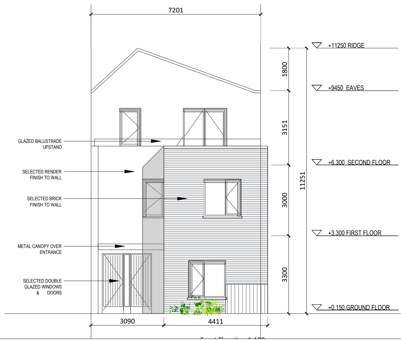
Duplex Type B1 Elevations & Section
